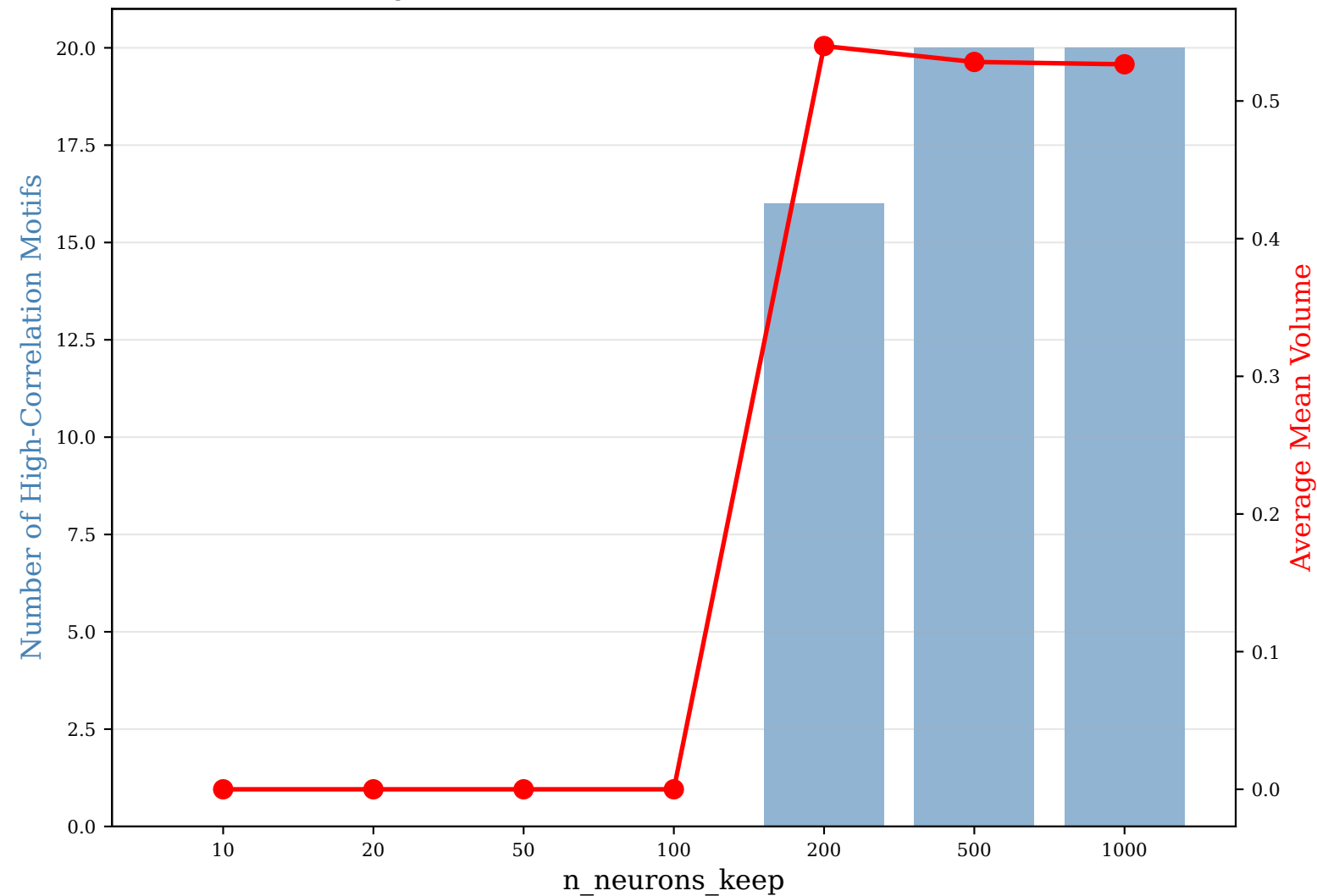
High-Correlation Motif Count and Volume Trends
